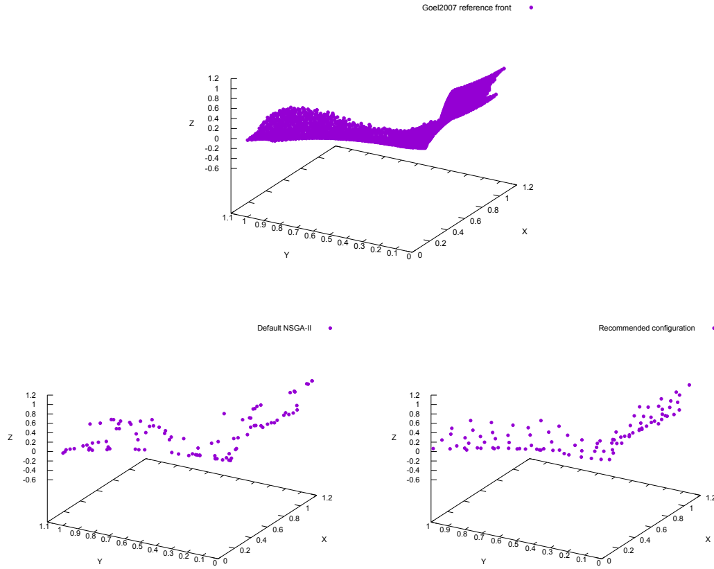
Figure 7.6: Reference front of Goel2007 (top), front obtained by NSGA-II with standard setting (bottom left), and front obtained by recommoonder (bottom right).
