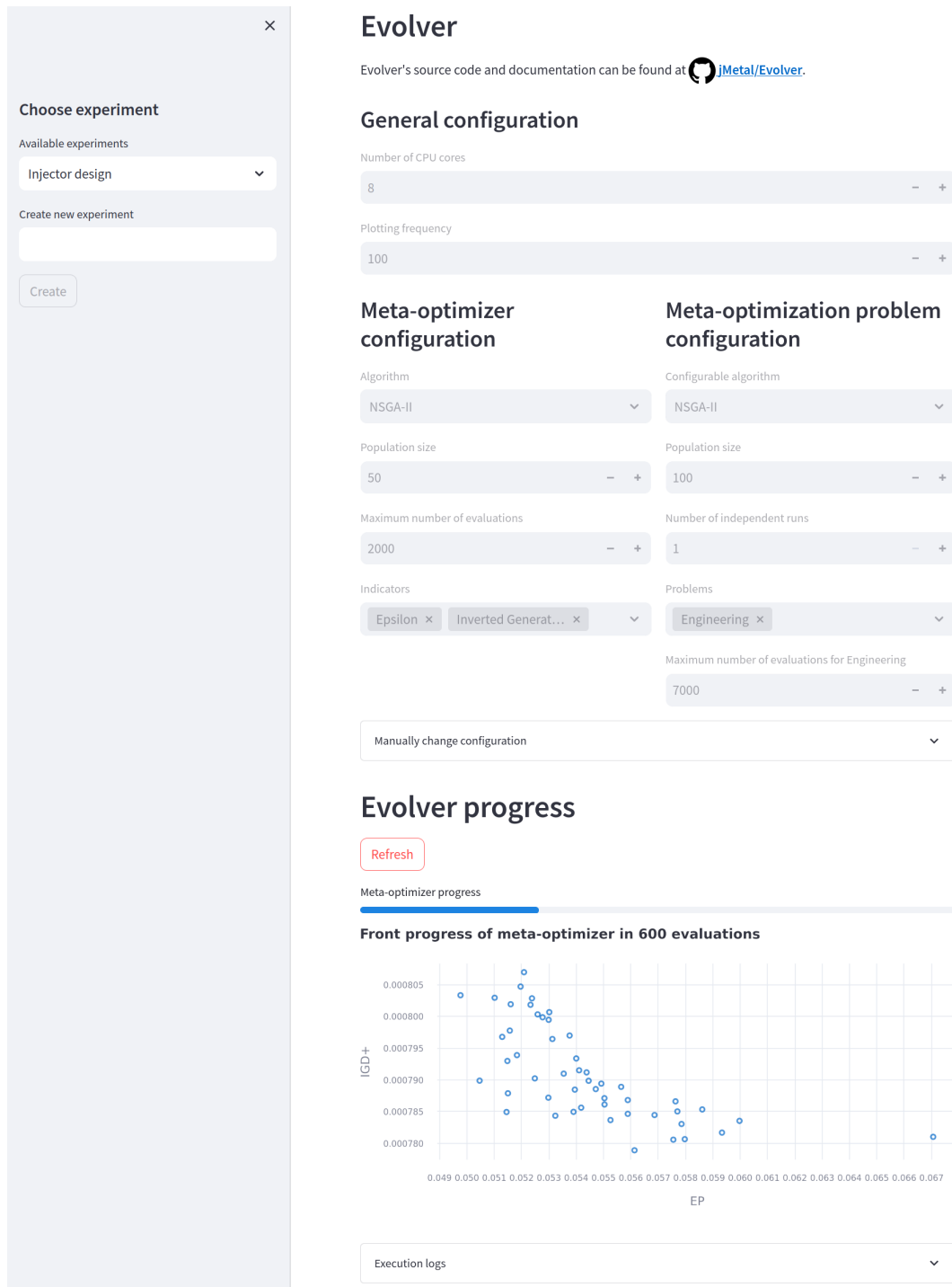
Figure 5.7: Evolver 's dashboard while executing the liquid-rocket single element injector design problem. The chart shows the population of the meta-optimizer after 600 function evaluations, which contains four non-dominated solutions.
