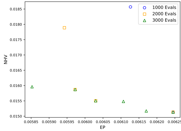
Figure 5.5: WFG problem family. Evolution of the front generated by the meta-optimizer.
