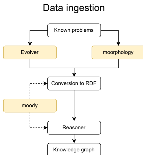
Figure 7.2: Ingestion pipeline for recommoender .
