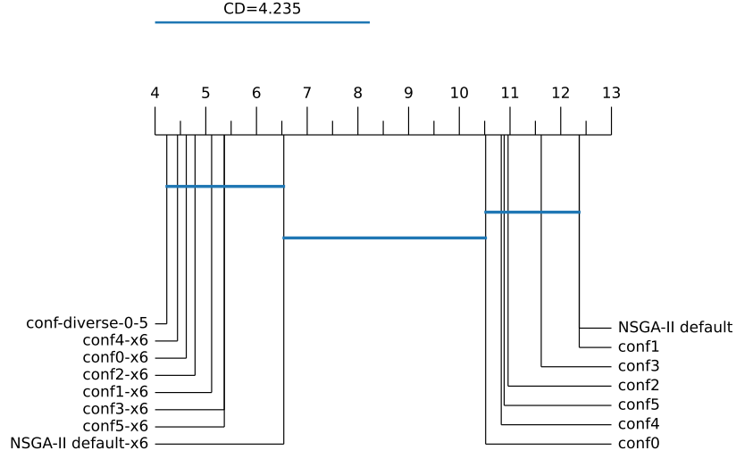
Figure 5.12: Critical distance plot ranking the obtained configurations and ensembles from the Quality-Diversity optimization process.
